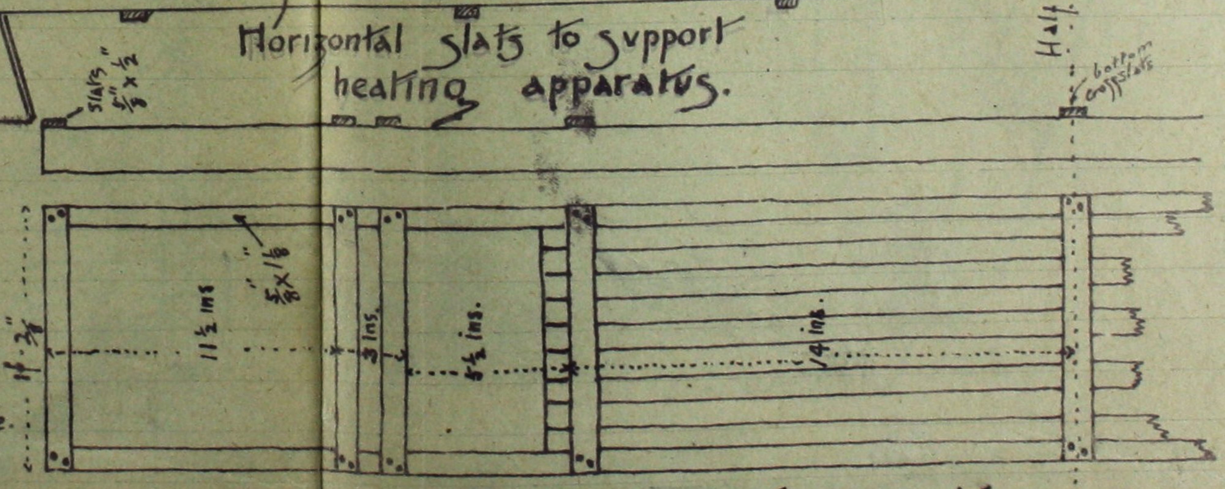
Sketch plan & elev. of heating apparatus support.
